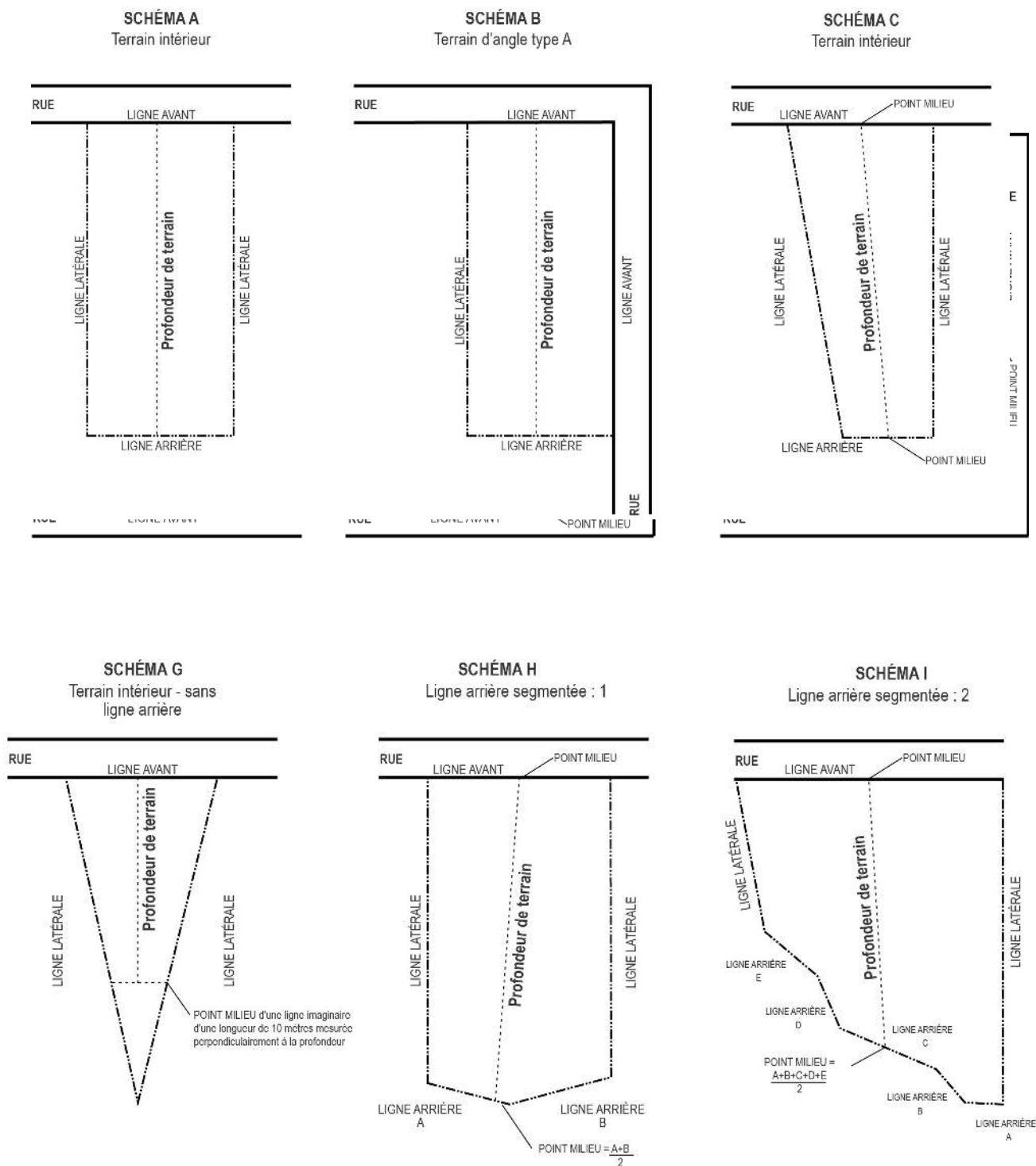
FIGURE 25 Dimensions de terrain
